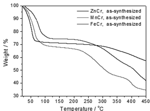
Figure 3. Thermogravimetric curves of \text{MCr} \cdot x\text{H}_2\text{O} .
