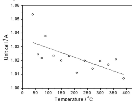
Figure 5. Temperature-dependent unit cell of \text{ZnCr} \cdot x\text{H}_2\text{O} from variable-temperature powder XRD data obtained under vacuum conditions.
